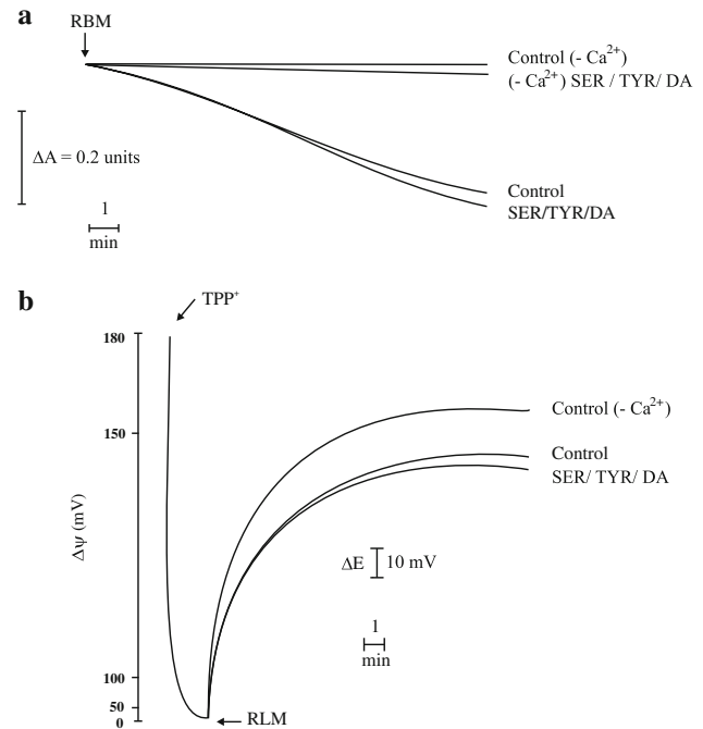
Fig. 5 Effect of monoamines on mitochondrial swelling ( a ) and \Delta\Psi drop ( b ) induced by \text{Ca}^{2+} in RBM. RBM were incubated in standard medium as described in “Materials and methods”. 100 \mu\text{M} \text{Ca}^{2+} was always present except when otherwise indicated; when reported the concentration of added monoamines was 100 \mu\text{M} . Downward deflections indicate mitochondrial swelling ( a ). 2 \mu\text{M} \text{TPP}^+ was used for \Delta\Psi measurements. \Delta E is the electrode potential ( b ). Traces are representative of six separate experiments
