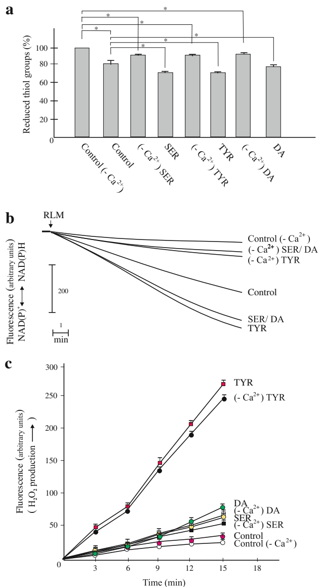
Fig. 4 Effects of calcium and monoamines on the redox state of sulfhydryl groups ( a ), and pyridine nucleotides ( b ), and hydrogen peroxide production ( c ) in RLM. Incubation conditions as described in “Materials and methods” with 50 \mu\text{M} \text{Ca}^{2+} and 100 \mu\text{M} monoamines present where indicated. The levels of sulfhydryl groups were measured after 12 min incubation and their total content was considered as 100%. Values are means of four experiments. *p < 0.05
